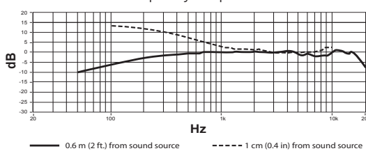
Frequency Response
